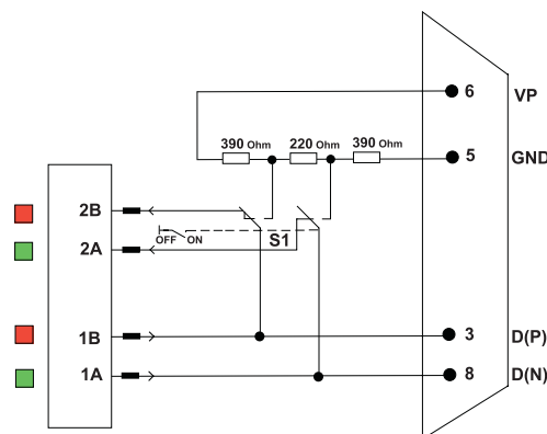
Functional diagram
