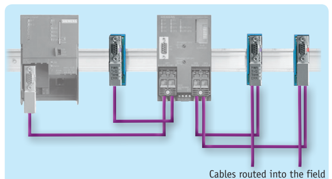
Fig. 9: Diagnostic repeater with three measuring points
