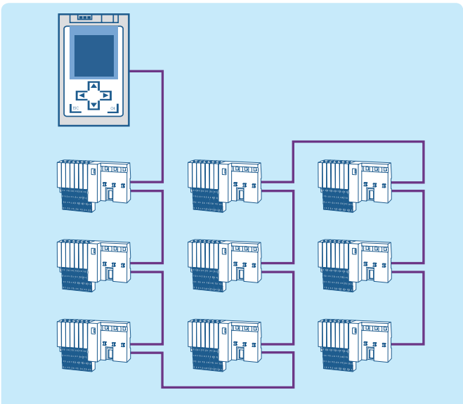
Fig. 18: Linear structure application example
