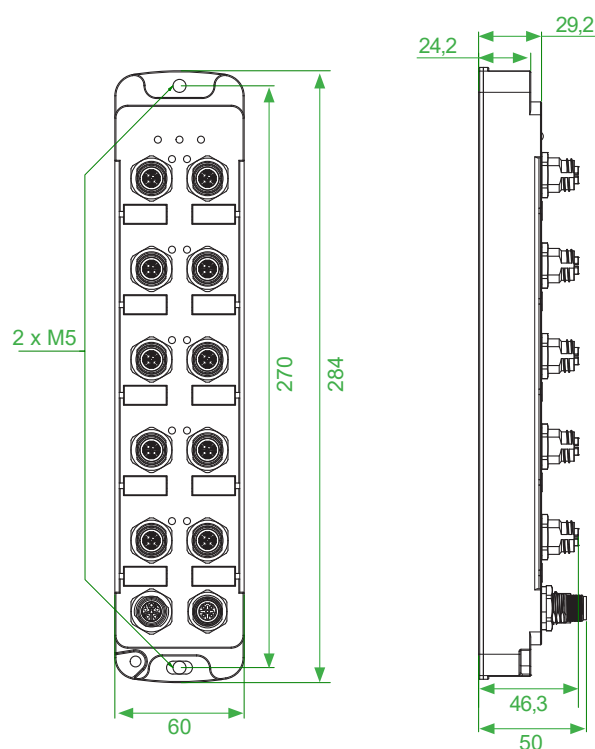
Dimensions (mm)
