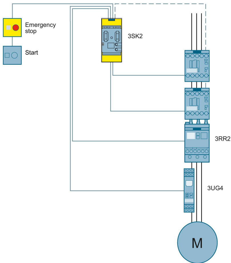
Figure 3-51 Safe current monitoring including Emergency Stop shutdown to SIL 2 or PL d with a 3SK2 safety relay and two current monitoring relays
