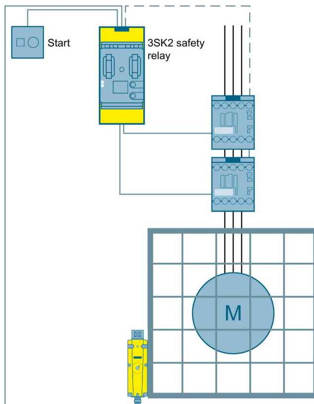
Figure 3-33 Protective door monitoring with tumbler to SIL 2 or PL d with a 3SK2 safety relay
