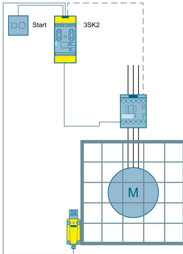
Figure 3-21 Protective door monitoring to SIL 1 or PL c with a 3SK2 safety relay
