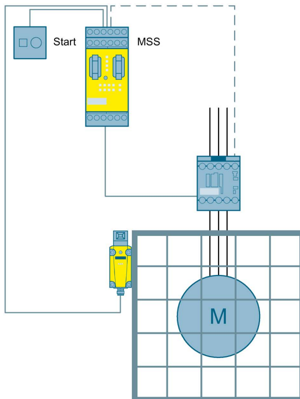
Figure 3-22 Protective door monitoring to SIL 1 or PL c with a Modular Safety System
