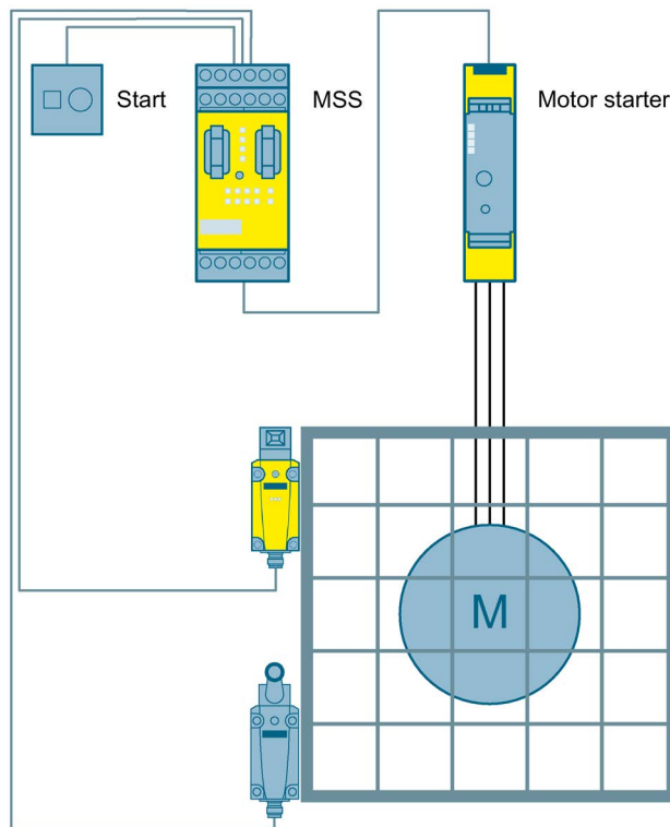
Figure 3-28 Protective door monitoring to SIL 3 or PL e with a fail-safe motor starter and a modular safety system
