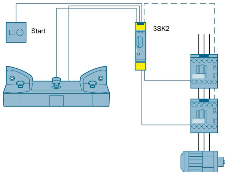
Figure 3-49 Two-hand operation to SIL 3 or PL e with a 3SK2 safety relay
