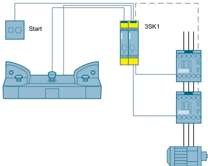
Figure 3-48 Two-hand operation to SIL 3 or PL e with a 3SK1 safety relay
