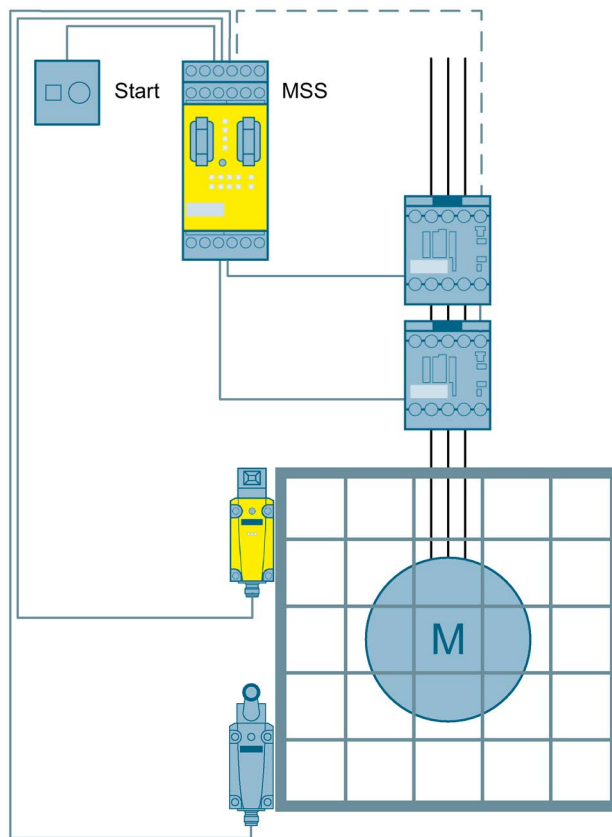
Figure 3-25 Protective door monitoring to SIL 3 or PL e with a Modular Safety System
