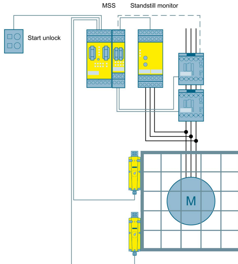
Figure 3-45 Safe standstill monitoring including protective door tumbler to SIL 3 or PL e with a Modular Safety System
