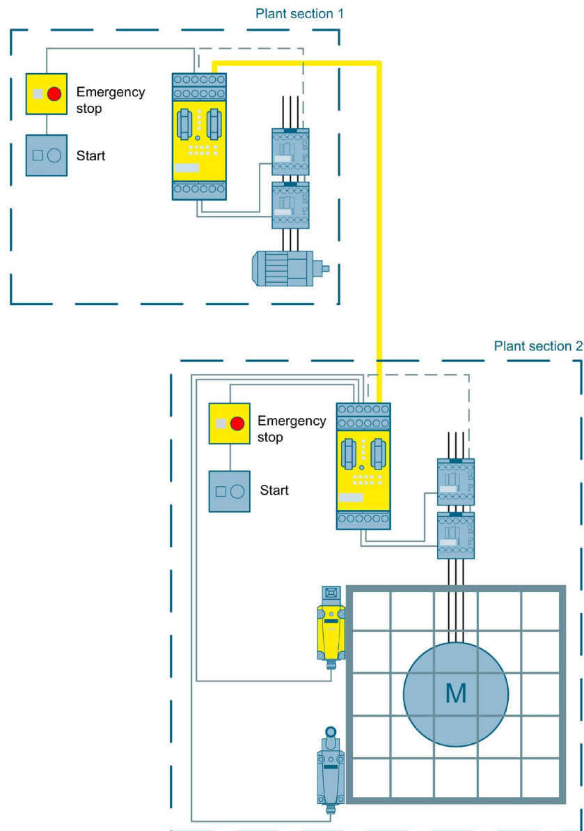
Figure 3-58 Safe slave-to-slave communication between several plant sections to SIL 3 or PL e via AS-i
