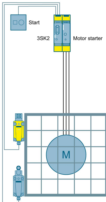
Figure 3-24 Protective door monitoring to SIL 3 or PL e with fail-safe motor starters and a 3SK2 safety relay
