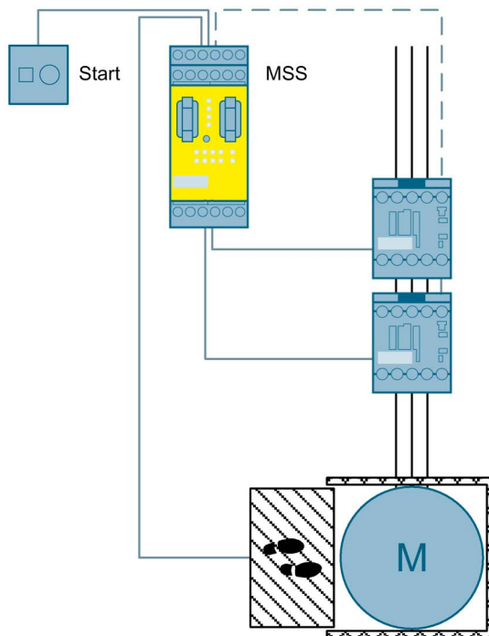
Figure 3-40 Access monitoring using a safety mat to SIL 3 or PL e with a Modular Safety System
