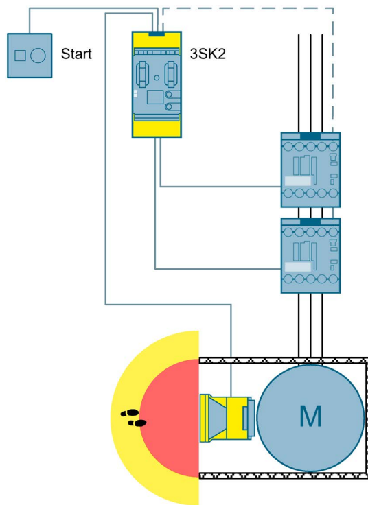
Figure 3-42 Area monitoring using a laser scanner to SIL 2 or PL d with a 3SK2 safety relay
