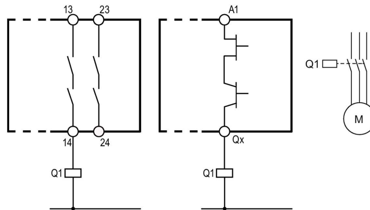
Figure 2-1 PL c acc. to ISO 13849-1, or SIL CL 1 acc. to IEC 62061
