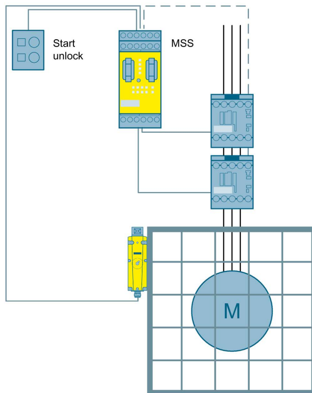
Figure 3-34 Protective door monitoring with tumbler to SIL 2 or PL d with a Modular Safety System
