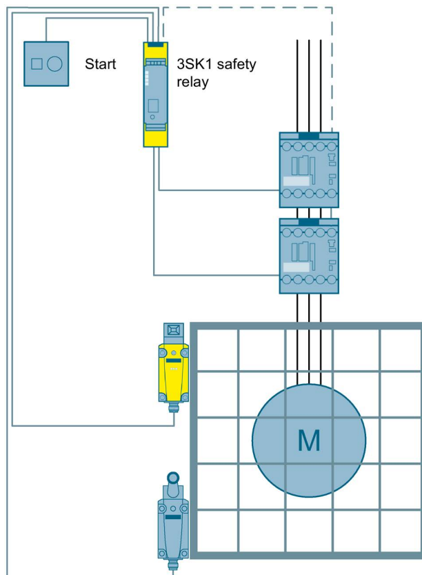
Figure 3-23 Protective door monitoring to SIL 3 or PL e with a 3SK1 safety relay
