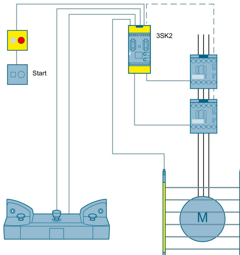
Figure 3-56 Access monitoring using a light curtain with two-hand operation and emergency stop to SIL 3 or PL e with a 3SK2 safety relay
