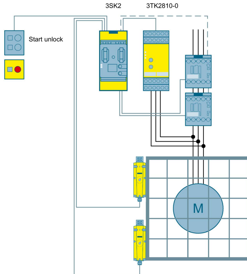
Figure 3-46 Safe standstill monitoring including protective door tumbler to SIL 3 or PL e with a 3SK2 safety relay
