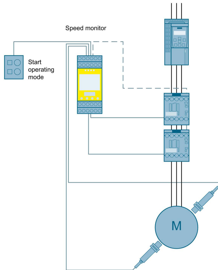
Figure 3-44 Safe speed monitoring to SIL 3 or PL e with a speed monitor
