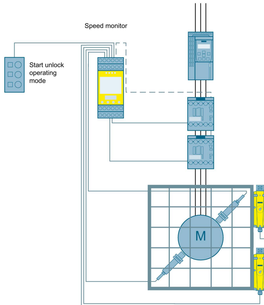
Figure 3-47 Safe speed monitoring, protective door monitoring and tumbler monitoring to SIL 3 or PL e with a speed monitor
