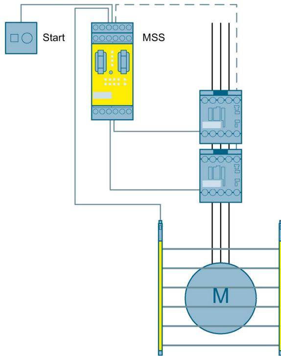
Figure 3-37 Access monitoring using a light curtain to SIL 3 or PL e with a Modular Safety System
