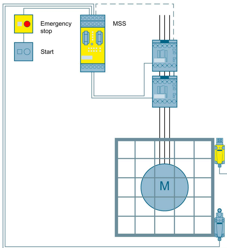
Figure 3-54 Emergency stop monitoring and protective door monitoring to SIL 3 or PL e with a Modular Safety System
