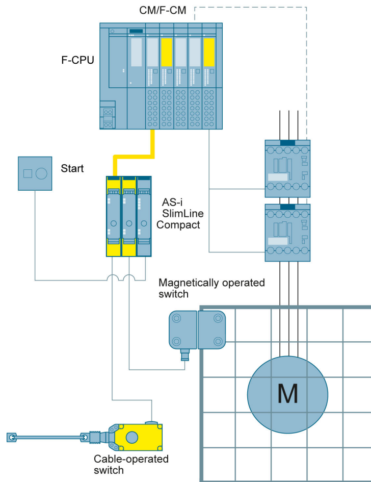
Figure 3-59 Protective door monitoring by means of magnetically-operated switches and emergency shutdown using cable-operated switch up to SIL3 or PL e by means of AS-i ET 200SP Master and AS-i SlimLine compact modules
