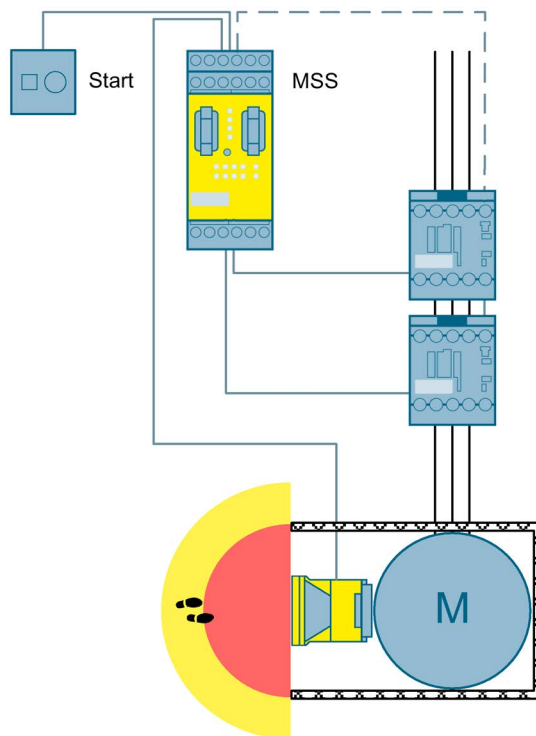
Figure 3-43 Area monitoring using a laser scanner to SIL 2 or PL d with a Modular Safety System
