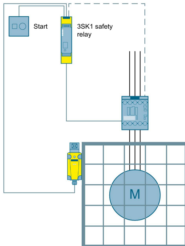
Figure 3-20 Protective door monitoring to SIL 1 or PL c with a 3SK1 safety relay
