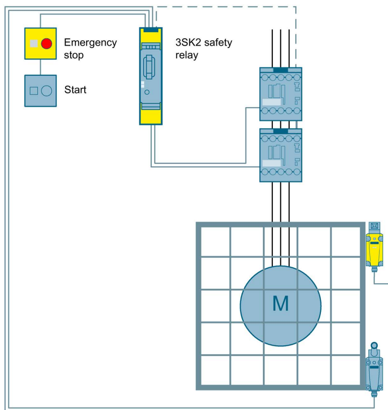
Figure 3-53 Emergency stop monitoring and protective door monitoring to SIL 3 or PL e with a 3SK2 safety relay
