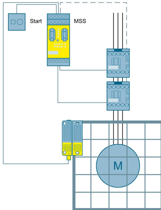
Figure 3-32 Protective door monitoring by means of RFID switch to SIL 3 or PL e with a Modular Safety System
