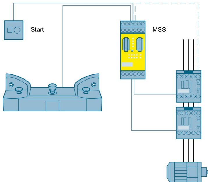
Figure 3-50 Two-hand operation to SIL 3 or PL e with a Modular Safety System
