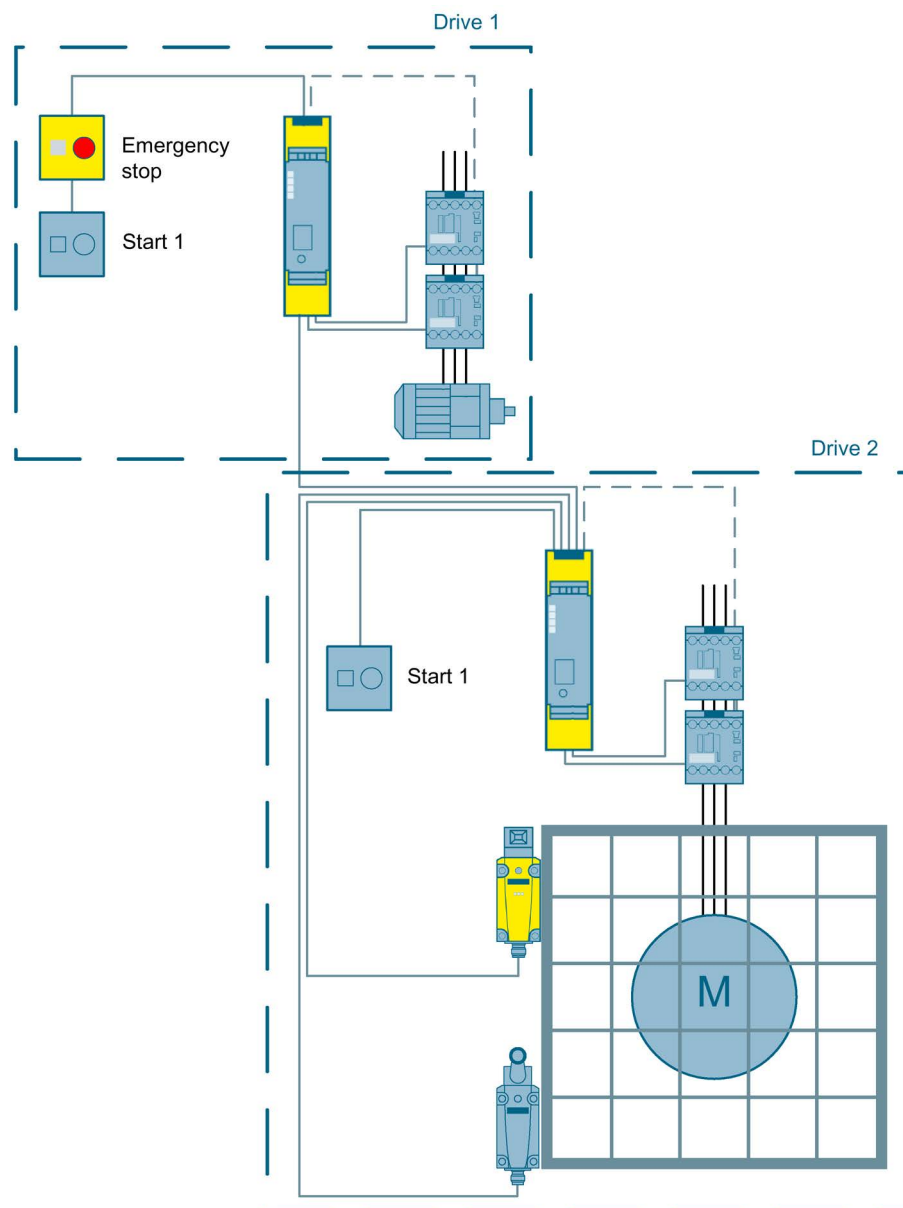
Figure 3-57 Cascading of 3SK1 safety relays to SIL 3 or PL e
