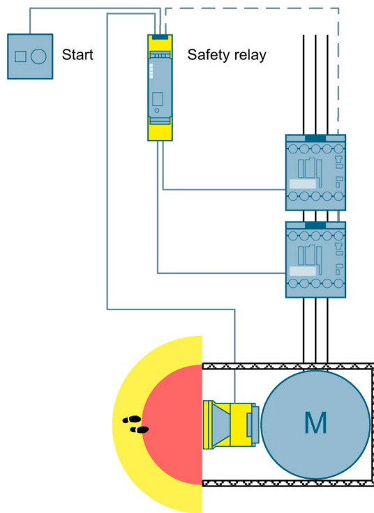
Figure 3-41 Area monitoring using a laser scanner to SIL 2 or PL d with a 3SK1 safety relay
